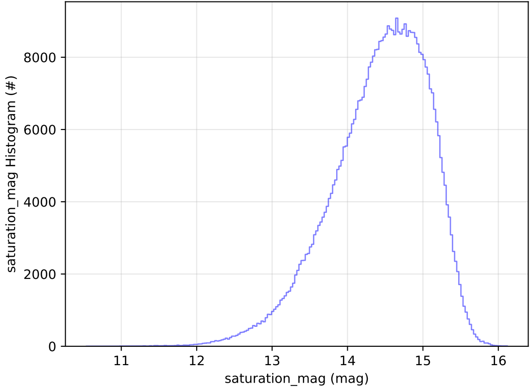
ddf_acor_sf25_lsf40_lsr20_v3.4_10yrs WFD i band: saturation_mag Histogram
