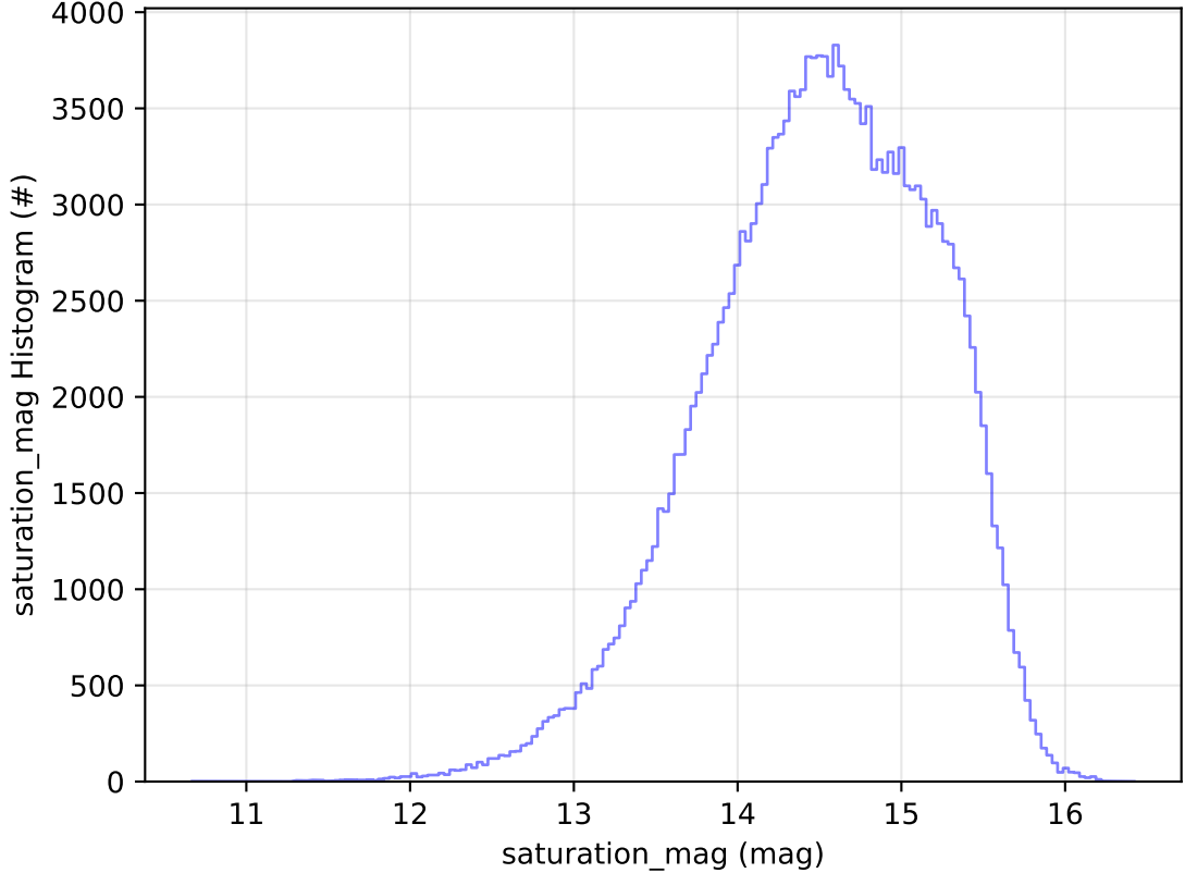
ddf_acor_sf25_lsf40_lsr20_v3.4_10yrs WFD g band: saturation_mag Histogram
