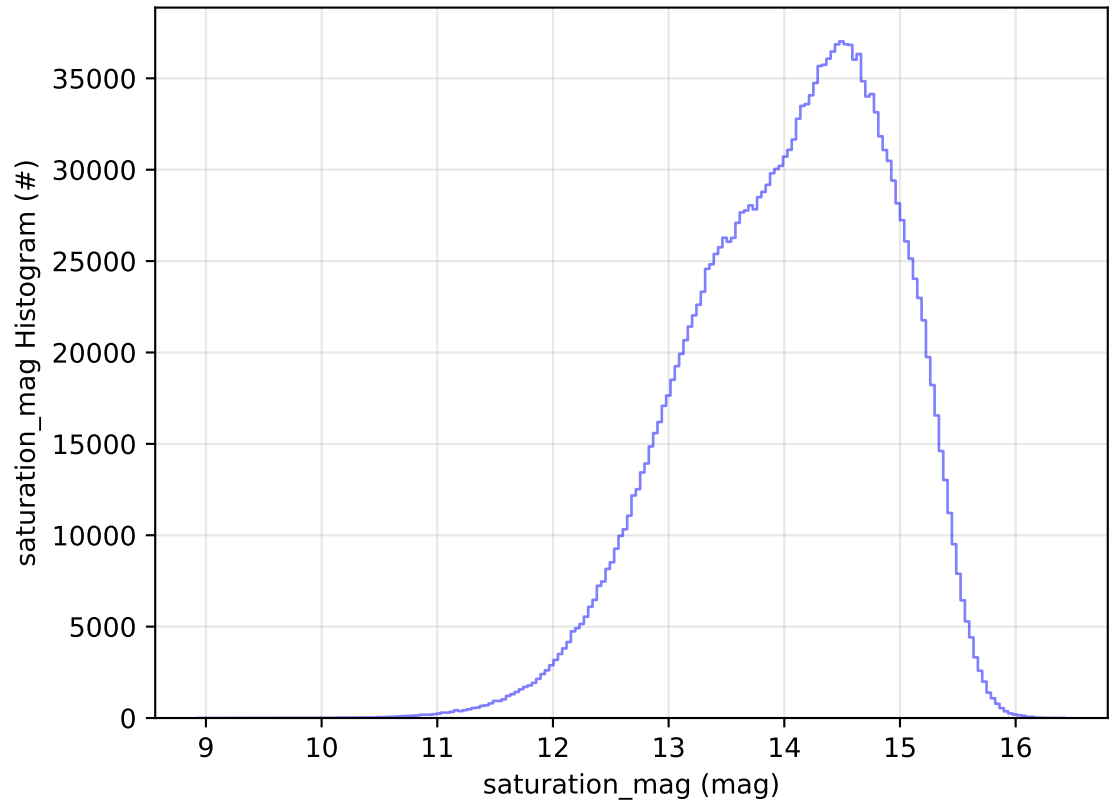
ddf_acor_sf25_lsf40_lsr20_v3.4_10yrs WFD all bands: saturation_mag Histogram
