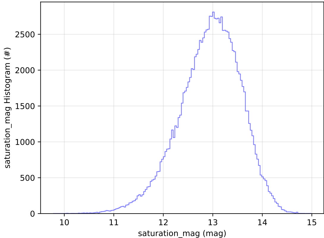
ddf_acor_sf25_lsf40_lsr20_v3.4_10yrs All sky u band: saturation_mag Histogram
