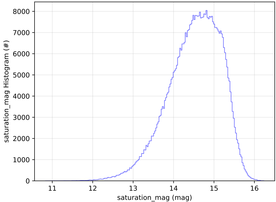
ddf_acor_sf25_lsf40_lsr20_v3.4_10yrs All sky r band: saturation_mag Histogram
