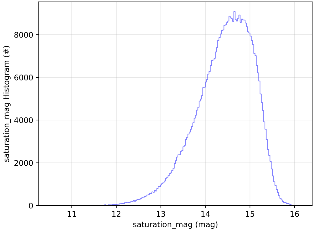
ddf_acor_sf25_lsf40_lsr20_v3.4_10yrs All sky i band: saturation_mag Histogram
