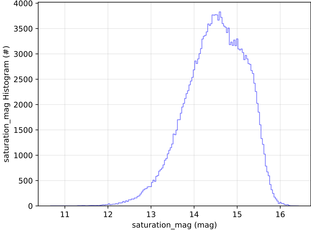
ddf_acor_sf25_lsf40_lsr20_v3.4_10yrs All sky g band: saturation_mag Histogram
