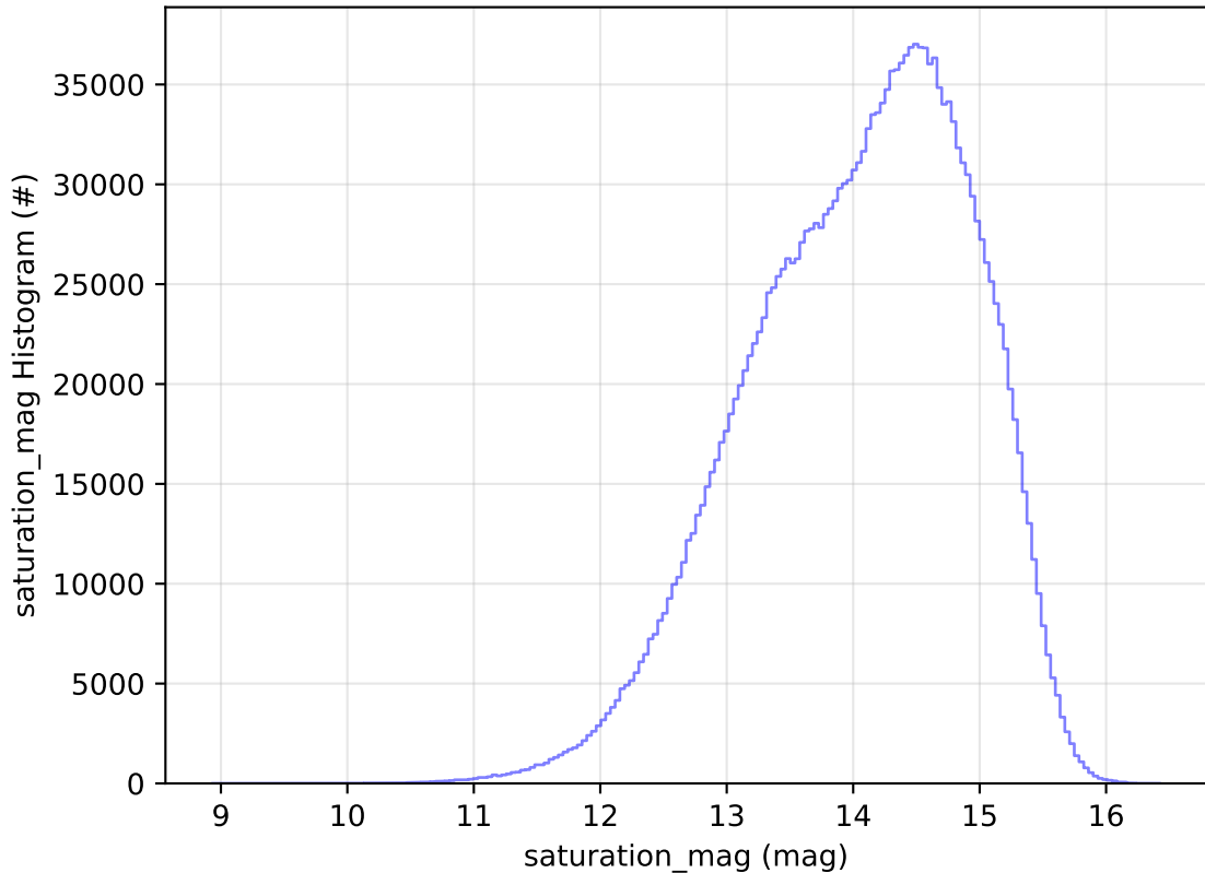
ddf_acor_sf25_lsf40_lsr20_v3.4_10yrs All sky all bands: saturation_mag Histogram
