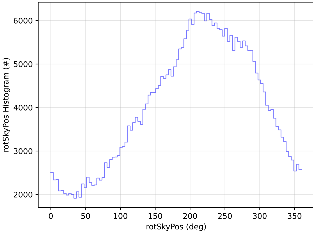
ddf_acor_sf25_lsf40_lsr20_v3.4_10yrs WFD y band: rotSkyPos Histogram
