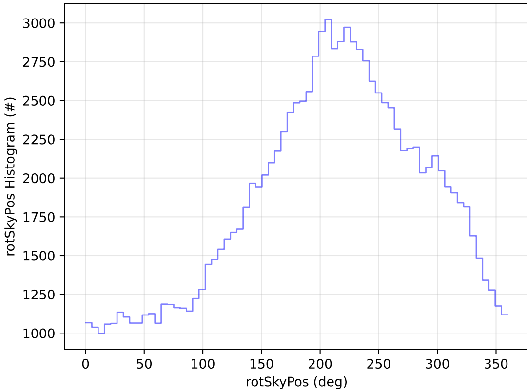
ddf_acor_sf25_lsf40_lsr20_v3.4_10yrs WFD u band: rotSkyPos Histogram
