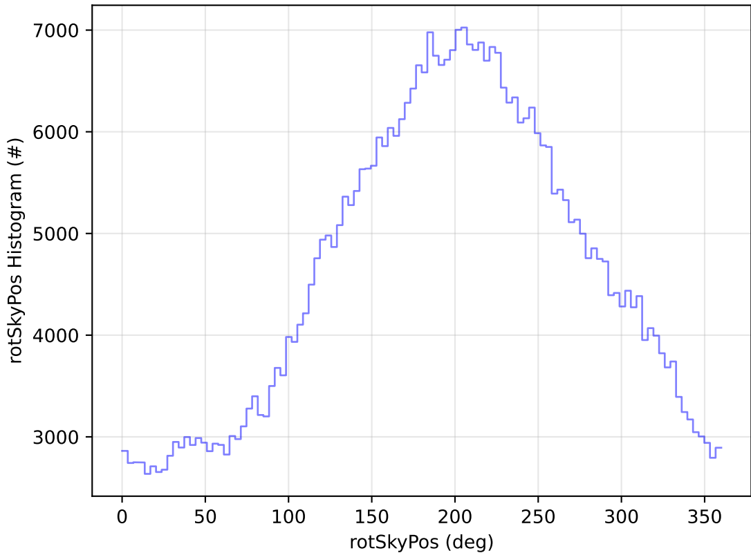
ddf_acor_sf25_lsf40_lsr20_v3.4_10yrs WFD r band: rotSkyPos Histogram
