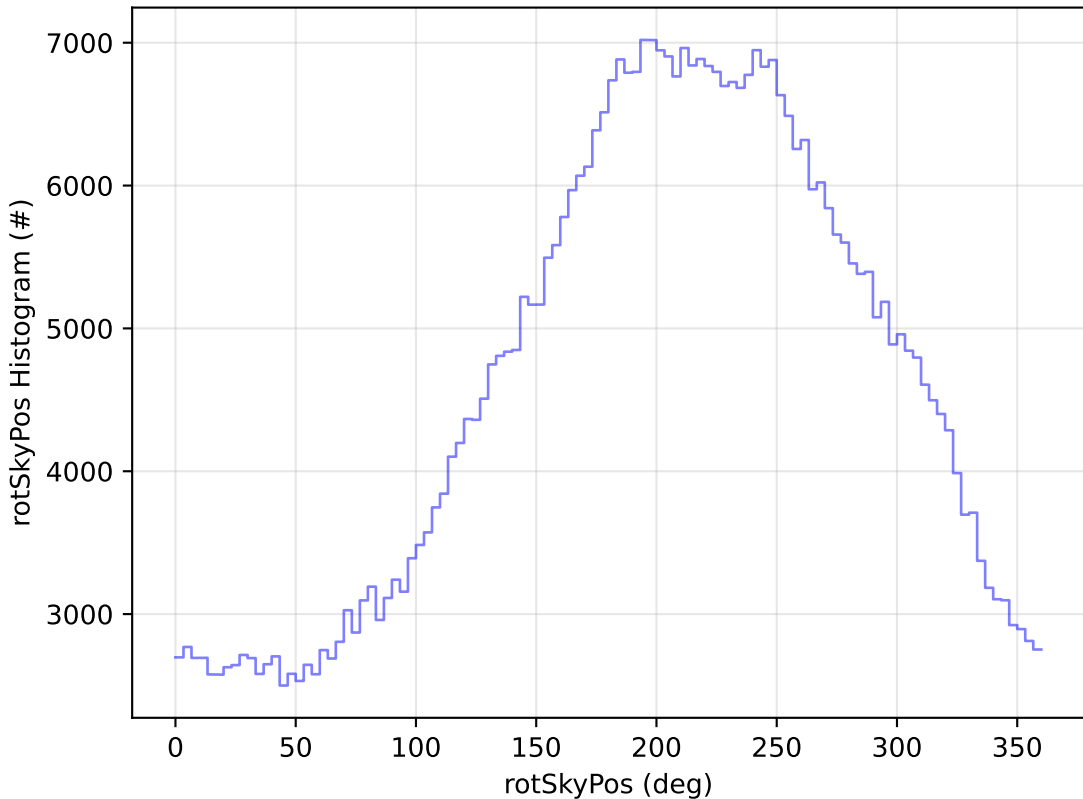
ddf_acor_sf25_lsf40_lsr20_v3.4_10yrs WFD i band: rotSkyPos Histogram
