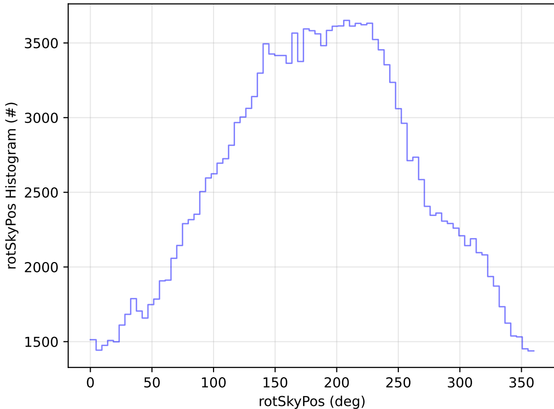
ddf_acor_sf25_lsf40_lsr20_v3.4_10yrs WFD g band: rotSkyPos Histogram
