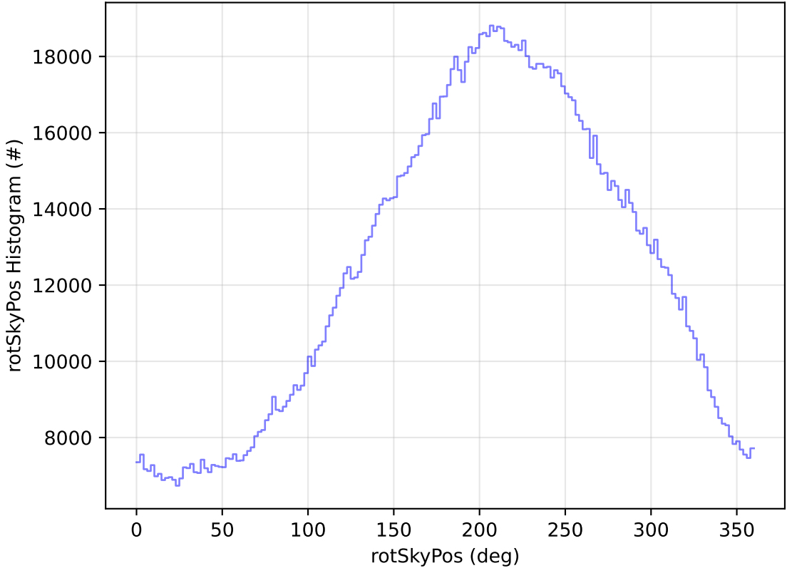
ddf_acor_sf25_lsf40_lsr20_v3.4_10yrs WFD all bands: rotSkyPos Histogram
