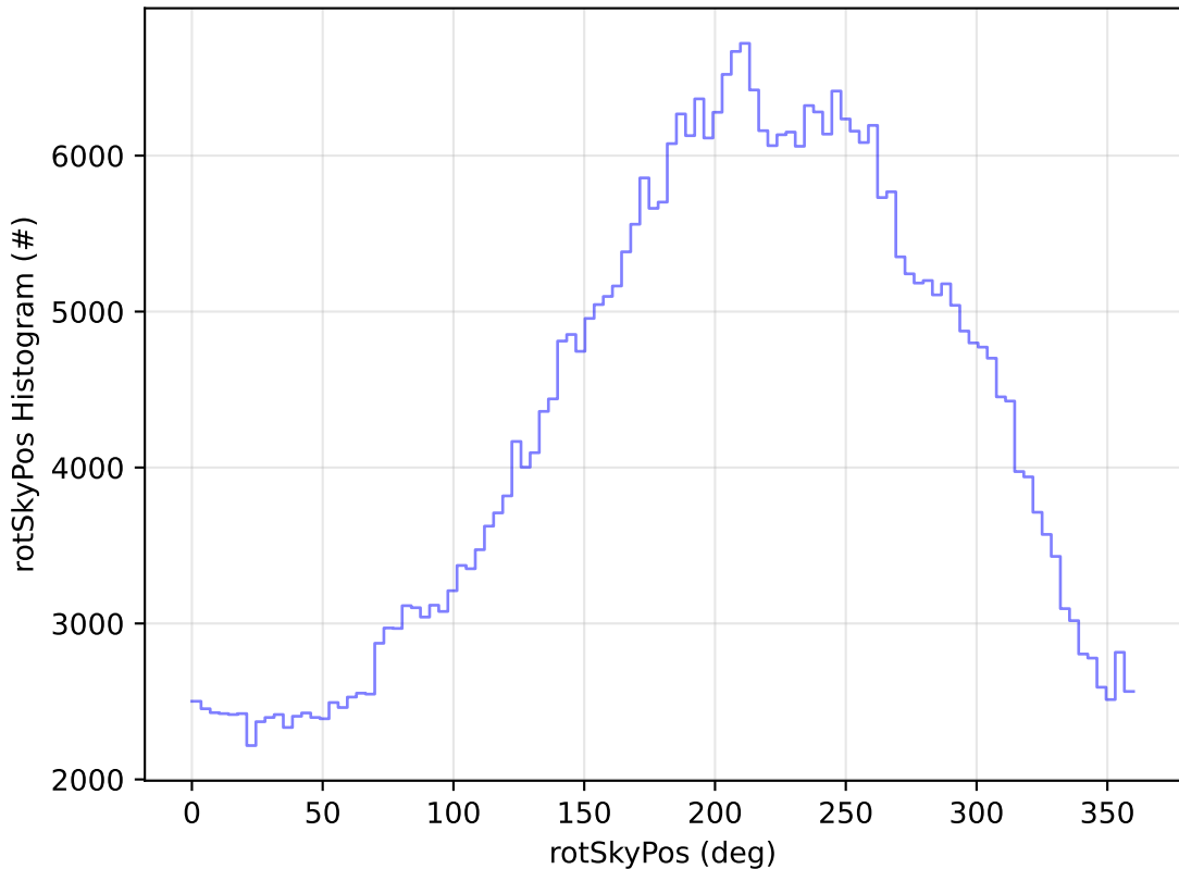
ddf_acor_sf25_lsf40_lsr20_v3.4_10yrs All sky z band: rotSkyPos Histogram
