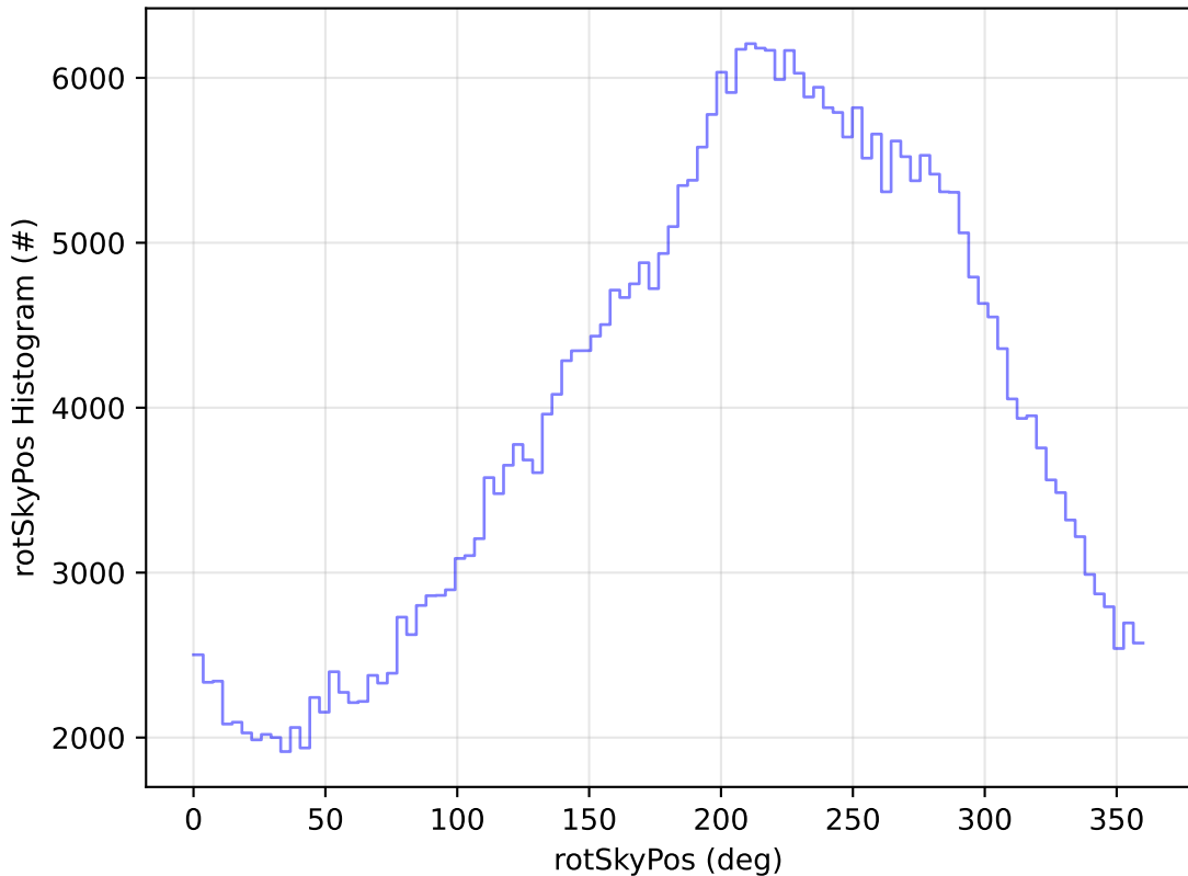
ddf_acor_sf25_lsf40_lsr20_v3.4_10yrs All sky y band: rotSkyPos Histogram
