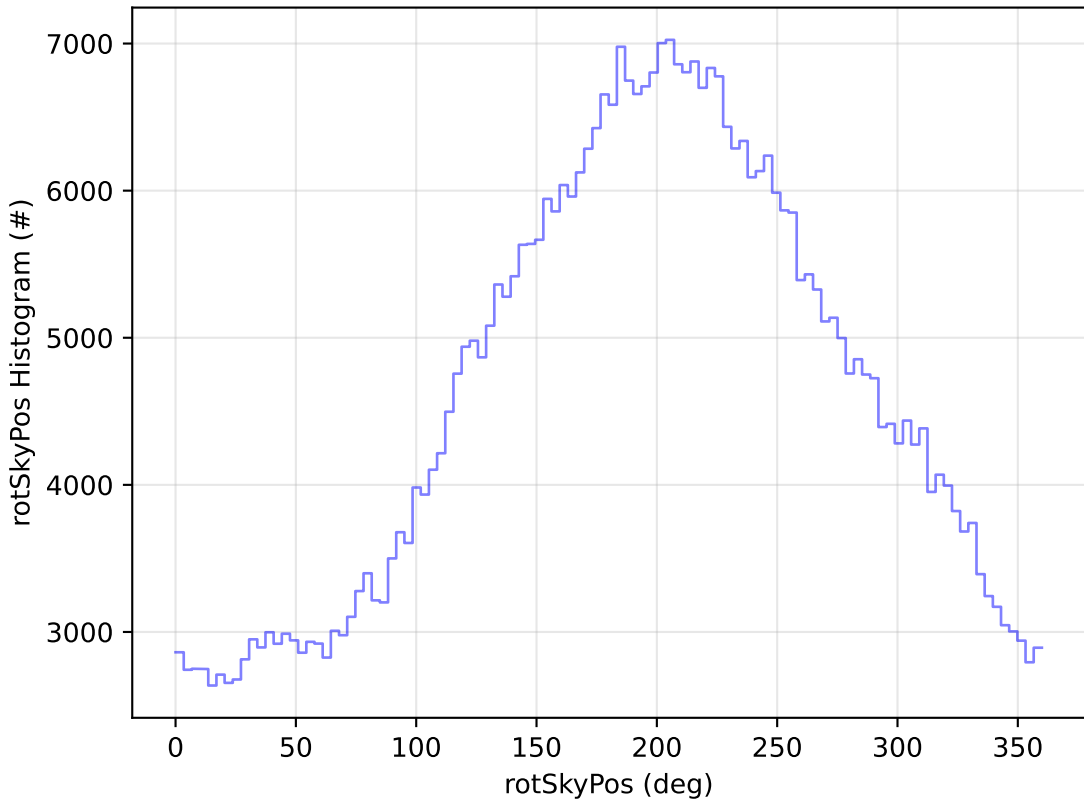
ddf_acor_sf25_ls40_lsr20_v3.4_10yrs All sky r band: rotSkyPos Histogram
