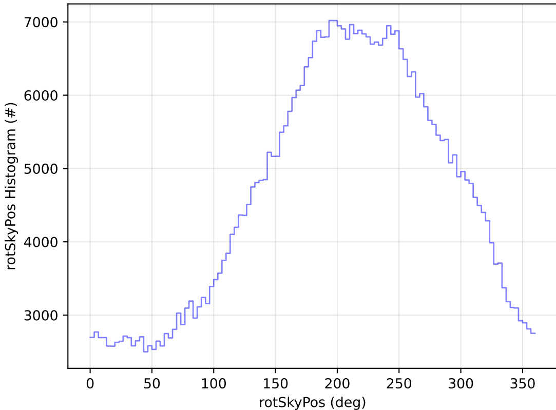
ddf_acor_sf25_lsf40_lsr20_v3.4_10yrs All sky i band: rotSkyPos Histogram
