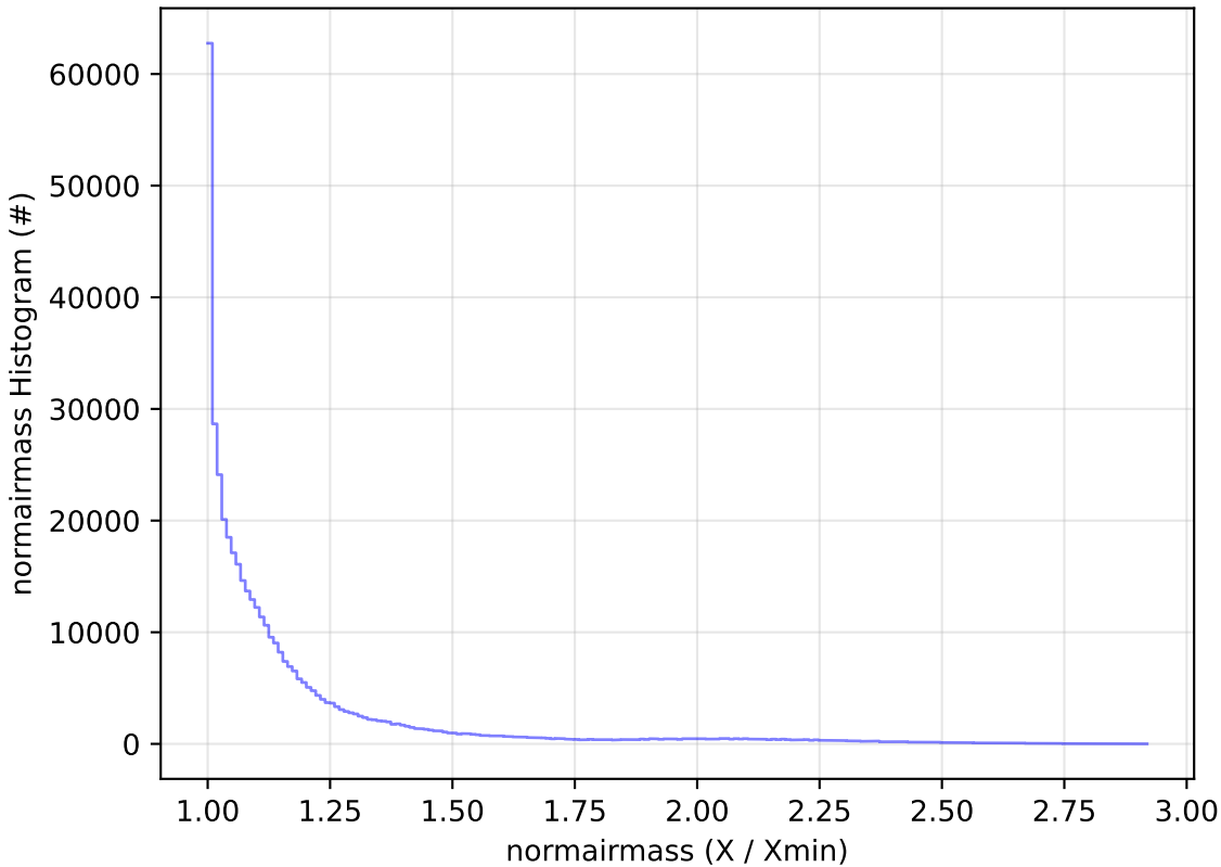
ddf_acor_sf25_lsf40_lsr20_v3.4_10yrs WFD z band: normairmass Histogram
