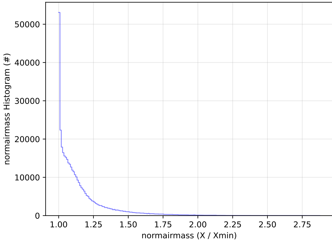
ddf_acor_sf25_lsf40_lsr20_v3.4_10yrs WFD y band: normairmass Histogram
