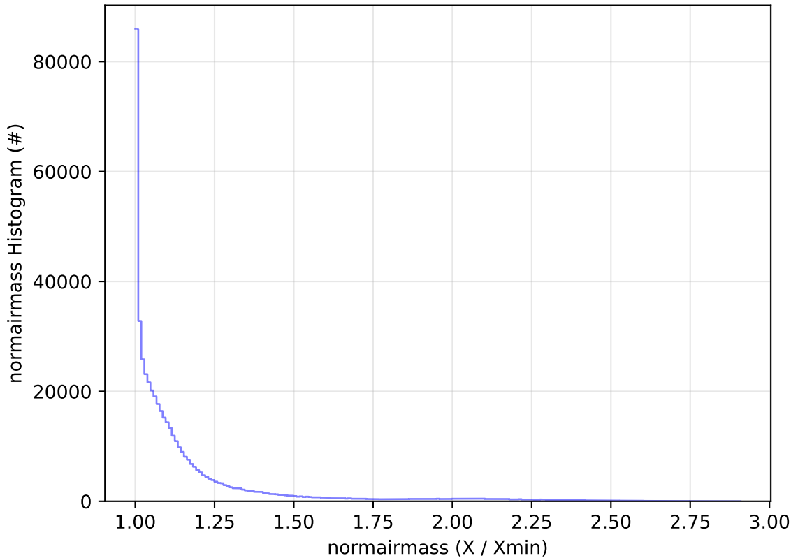
ddf_acor_sf25_lsf40_lsr20_v3.4_10yrs WFD i band: normairmass Histogram
