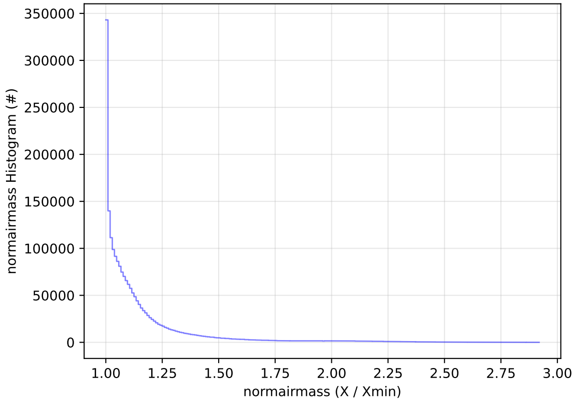
ddf_acor_sf25_lsf40_lsr20_v3.4_10yrs WFD all bands: normairmass Histogram
