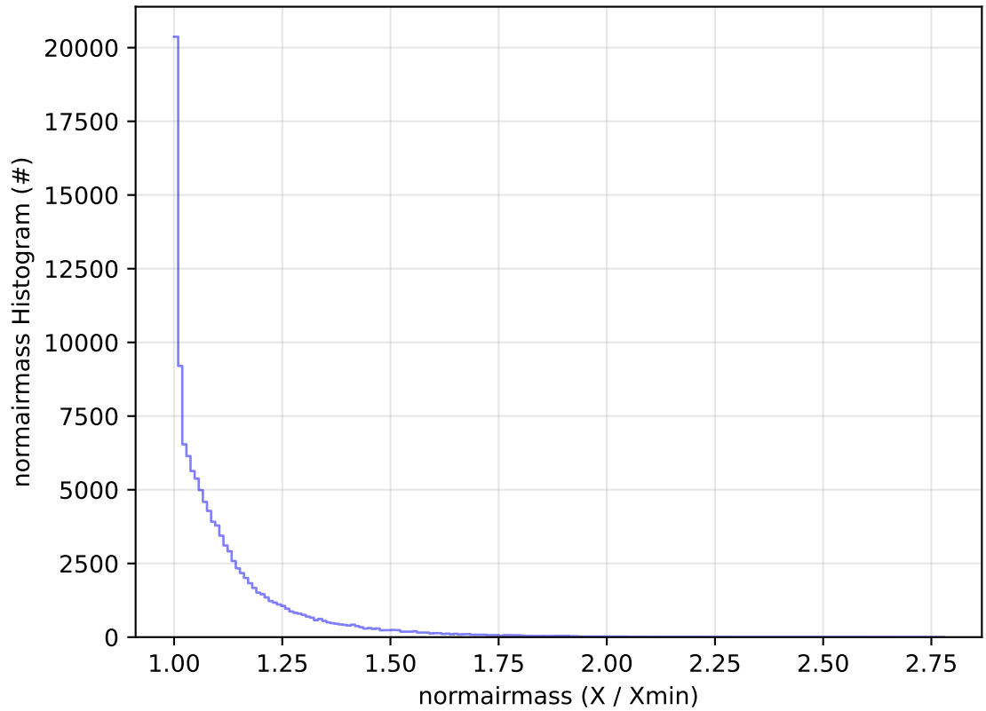
ddf_acor_sf25_lsf40_lsr20_v3.4_10yrs All sky u band: normairmass Histogram
