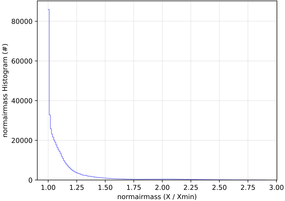
ddf_acor_sf25_lsf40_lsr20_v3.4_10yrs All sky i band: normairmass Histogram
