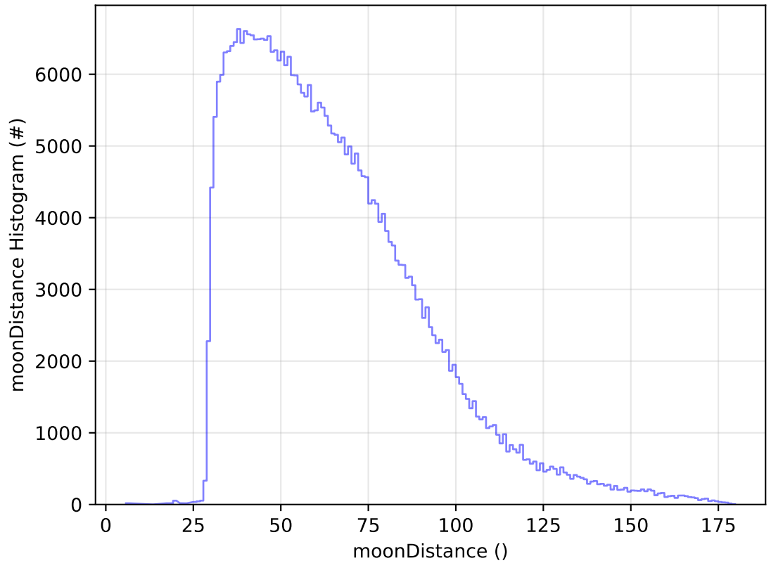
ddf_acor_sf25_lsf40_lsr20_v3.4_10yrs WFD y band: moonDistance Histogram
