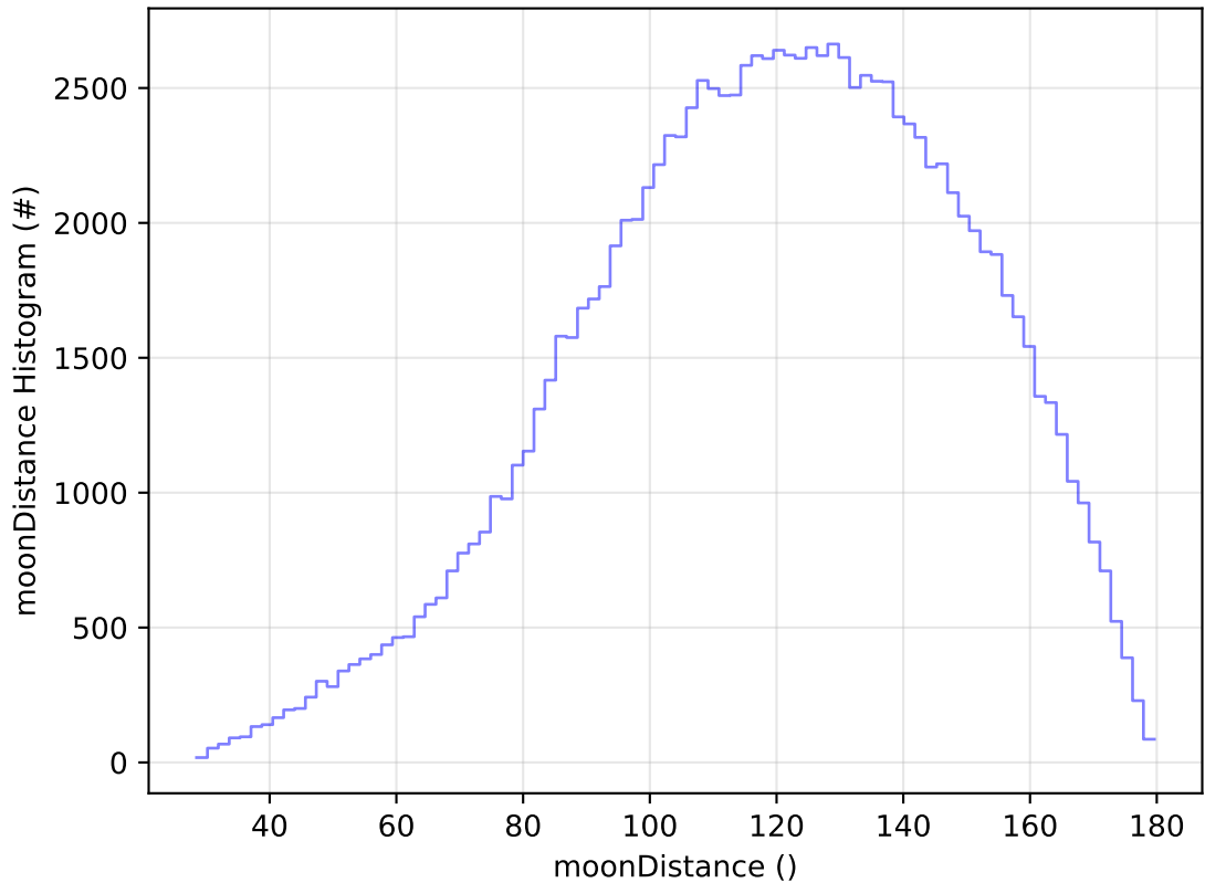
ddf_acor_sf25_lsf40_lsr20_v3.4_10yrs WFD u band: moonDistance Histogram
