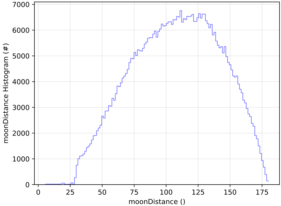
ddf_acor_sf25_lsf40_lsr20_v3.4_10yrs WFD r band: moonDistance Histogram
