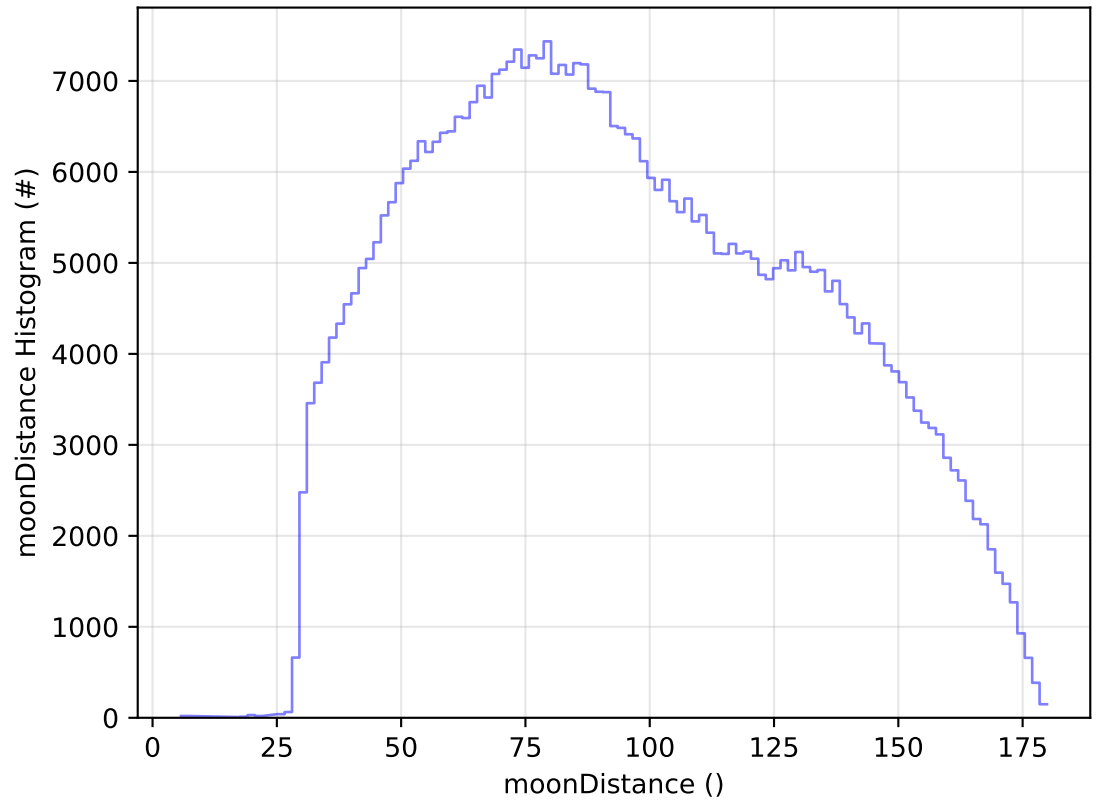
ddf_acor_sf25_lsf40_lsr20_v3.4_10yrs WFD i band: moonDistance Histogram
