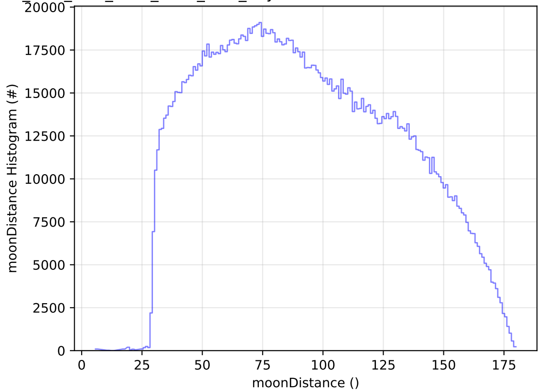
ddf_acor_sf25_lsf40_lsr20_v3.4_10yrs WFD all bands: moonDistance Histogram
