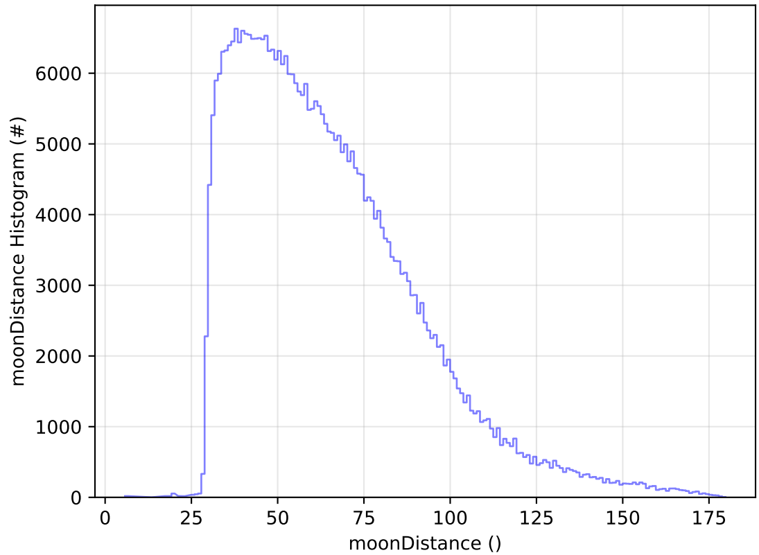
ddf_acor_sf25_lsf40_lsr20_v3.4_10yrs All sky y band: moonDistance Histogram
