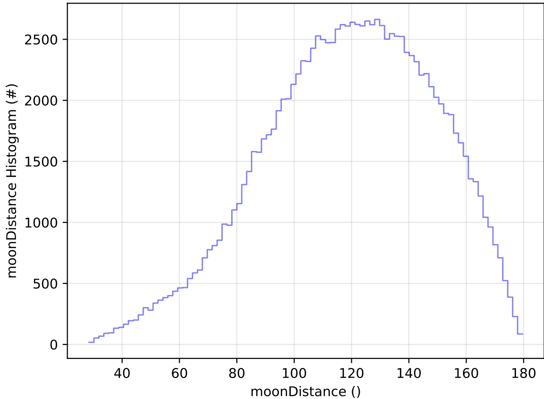
ddf_acor_sf25_lsf40_lsr20_v3.4_10yrs All sky u band: moonDistance Histogram
