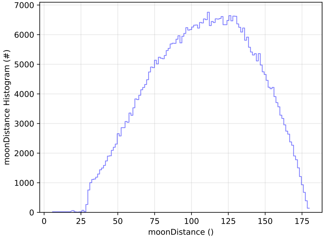
ddf_acor_sf25_lsf40_lsr20_v3.4_10yrs All sky r band: moonDistance Histogram
