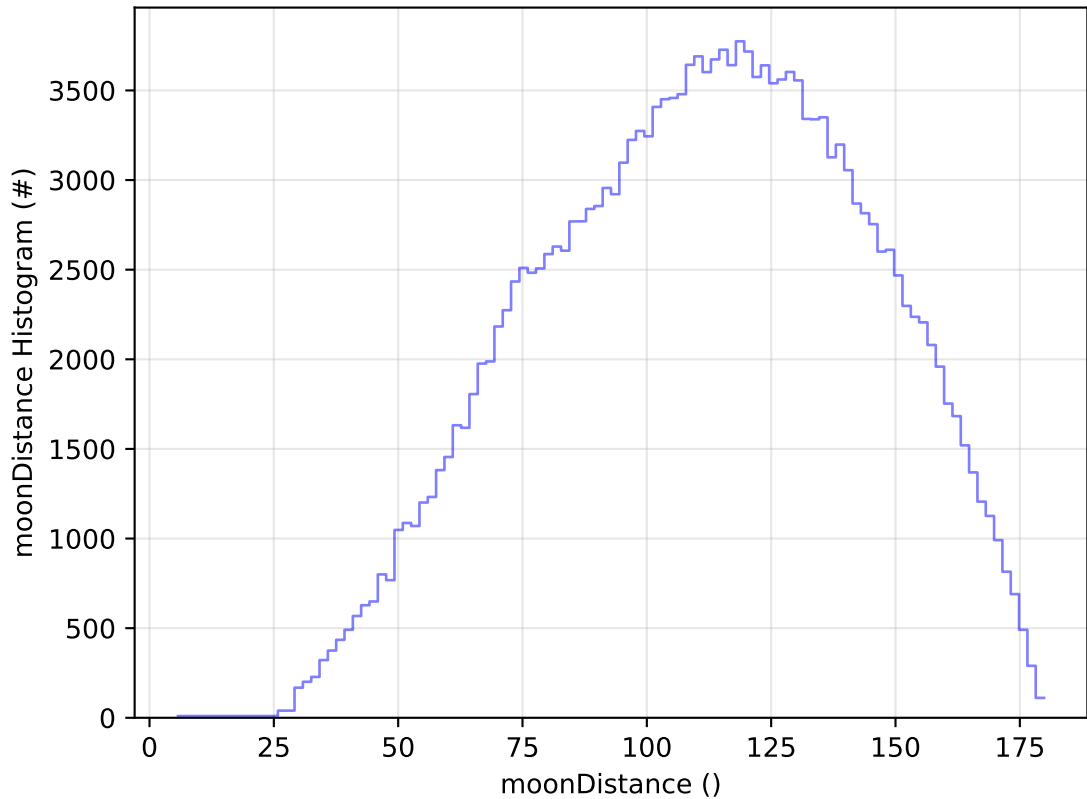
ddf_acor_sf25_lsf40_lsr20_v3.4_10yrs All sky g band: moonDistance Histogram
