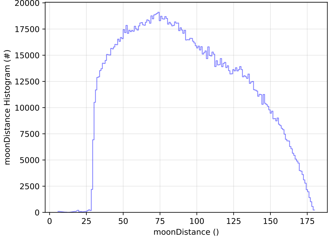
ddf_acor_sf25_lsf40_lsr20_v3.4_10yrs All sky all bands: moonDistance Histogram
