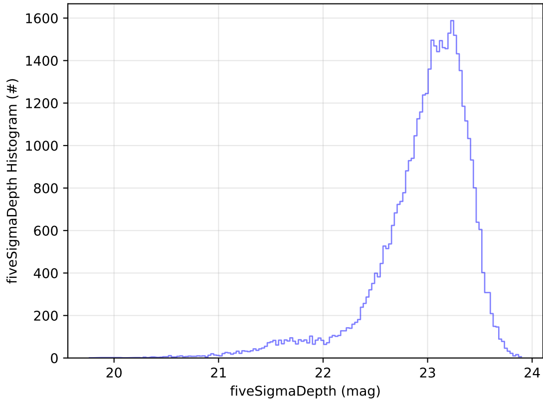
ddf_acor_sf25_lsf40_lsr20_v3.4_10yrs Yr 1 z band: fiveSigmaDepth Histogram
