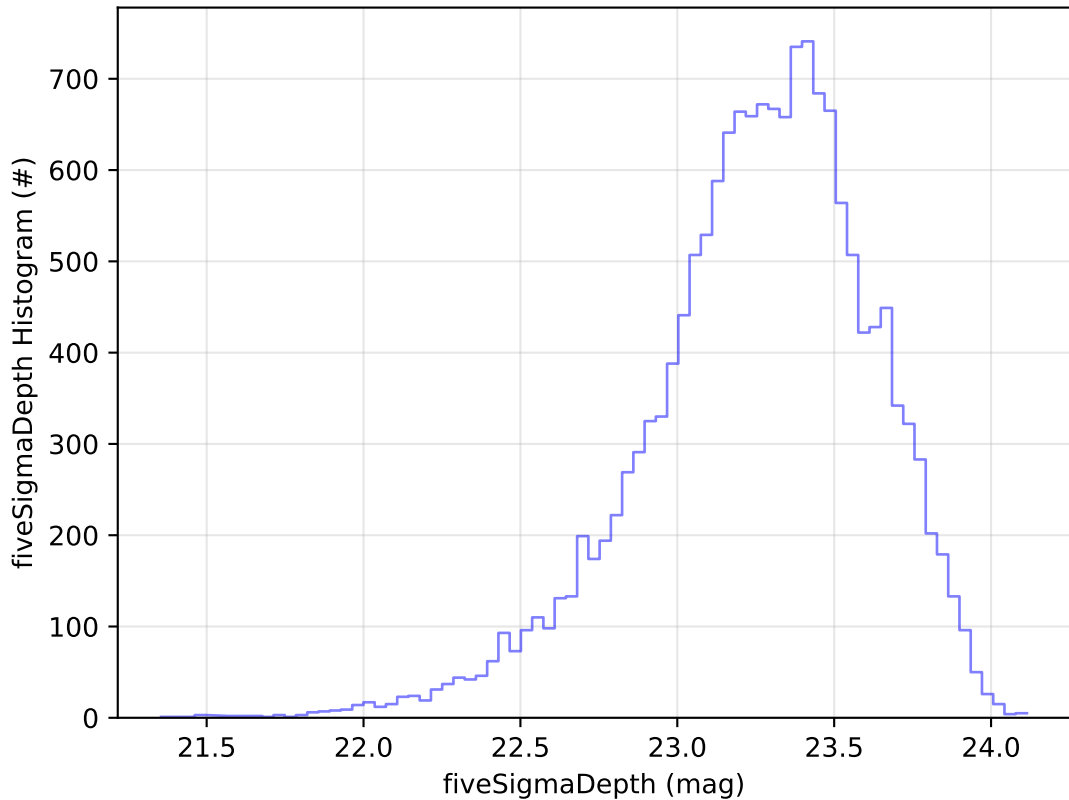
ddf_acor_sf25_lsf40_lsr20_v3.4_10yrs Yr 1 u band: fiveSigmaDepth Histogram
