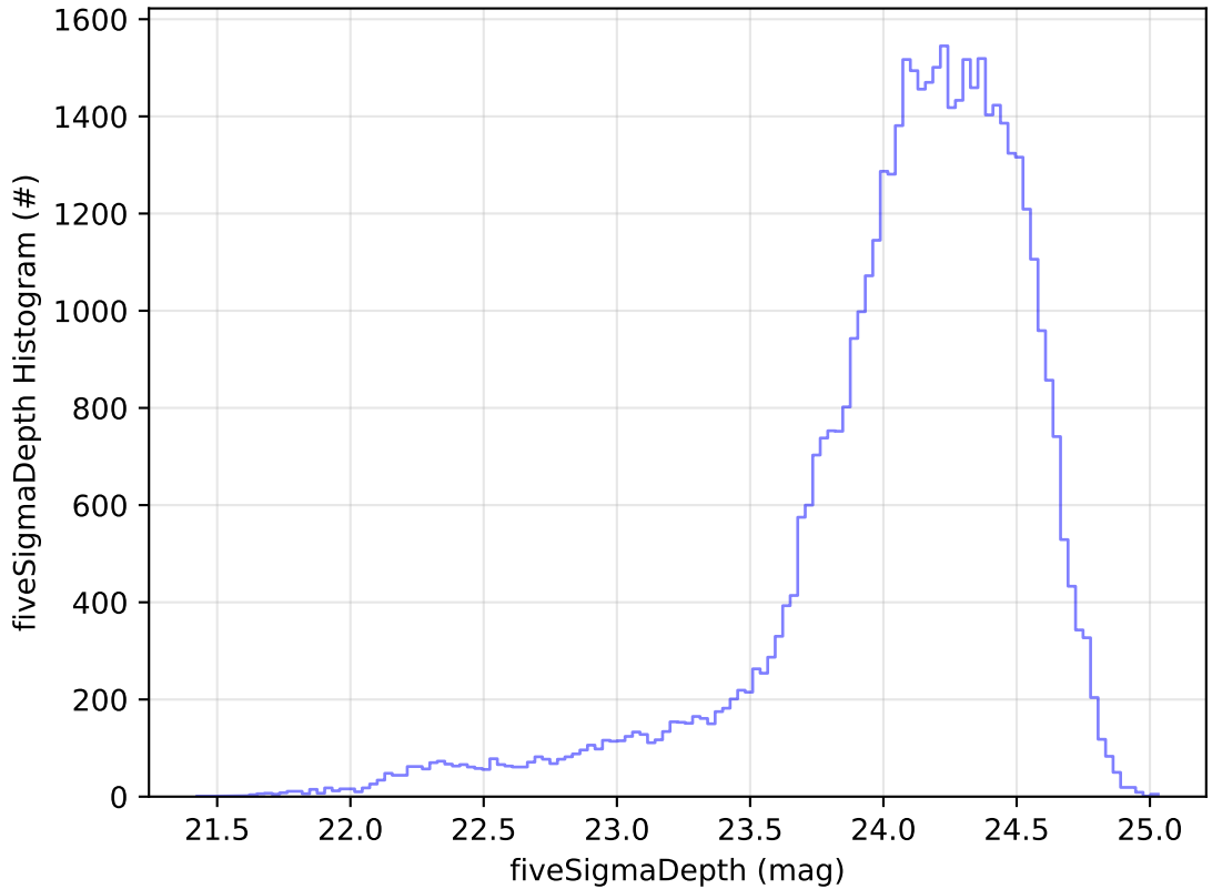
ddf_acor_sf25_lsf40_lsr20_v3.4_10yrs Yr 1 r band: fiveSigmaDepth Histogram
