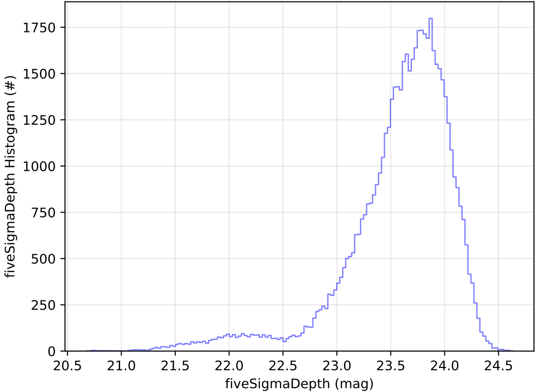
ddf_acor_sf25_lsf40_lsr20_v3.4_10yrs Yr 1 i band: fiveSigmaDepth Histogram
