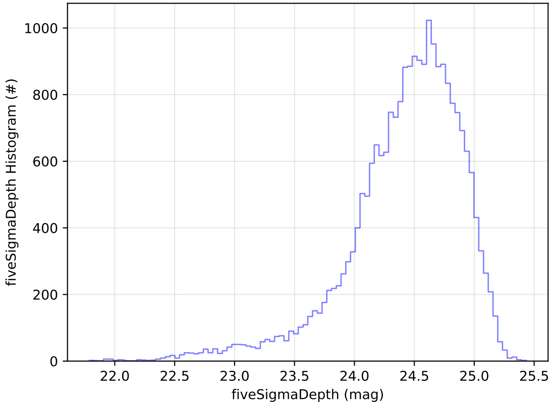
ddf_acor_sf25_lsf40_lsr20_v3.4_10yrs Yr 1 g band: fiveSigmaDepth Histogram
