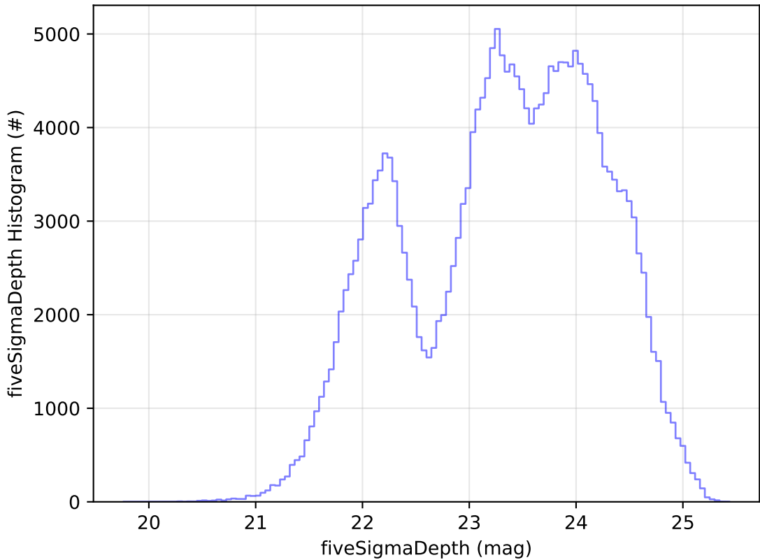
ddf_acor_sf25_lsf40_lsr20_v3.4_10yrs Yr 1 all bands: fiveSigmaDepth Histogram
