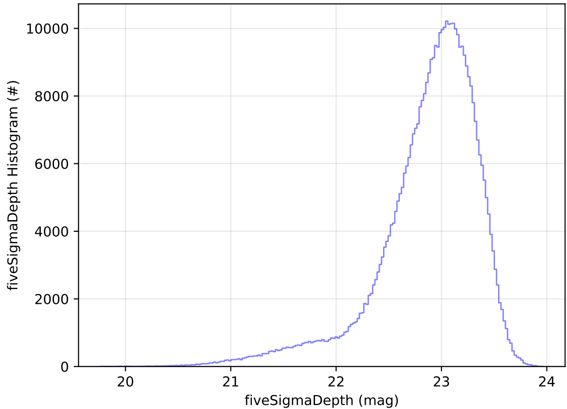
ddf_acor_sf25_lsf40_lsr20_v3.4_10yrs WFD z band: fiveSigmaDepth Histogram
