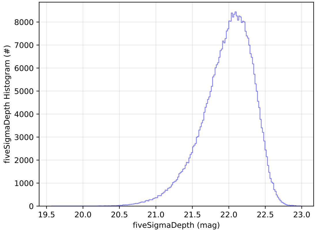
ddf_acor_sf25_lsf40_lsr20_v3.4_10yrs WFD y band: fiveSigmaDepth Histogram
