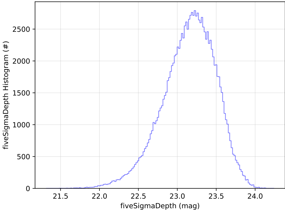
ddf_acor_sf25_lsf40_lsr20_v3.4_10yrs WFD u band: fiveSigmaDepth Histogram
