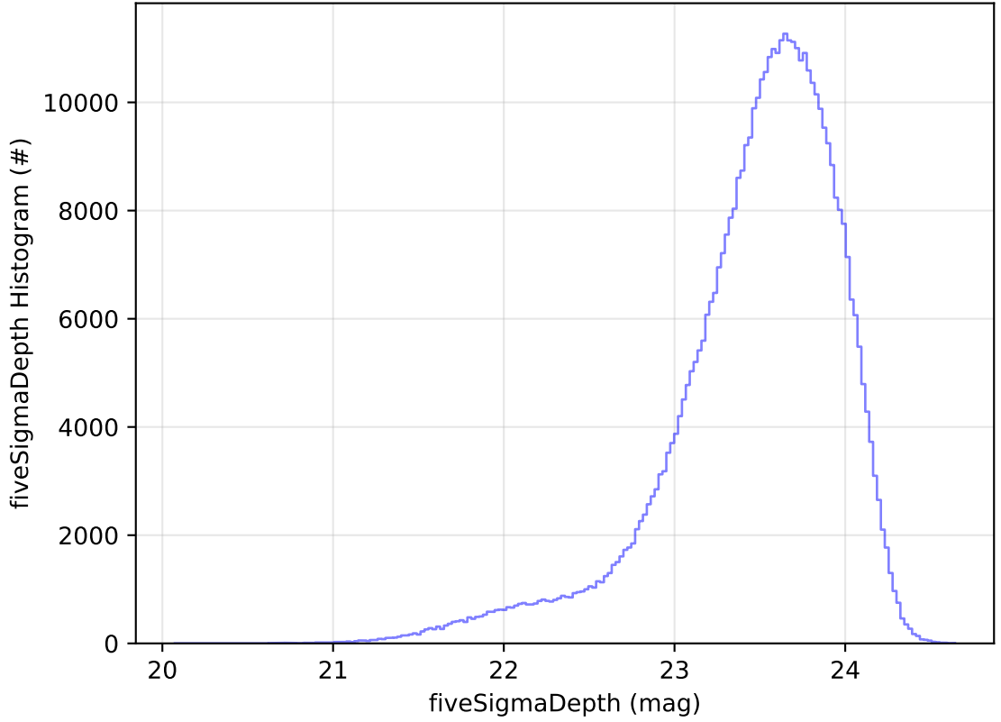
ddf_acor_sf25_lsf40_lsr20_v3.4_10yrs WFD i band: fiveSigmaDepth Histogram
