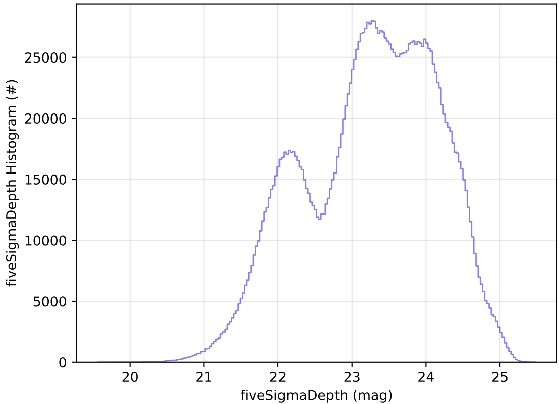
ddf_acor_sf25_lsf40_lsr20_v3.4_10yrs WFD all bands: fiveSigmaDepth Histogram
