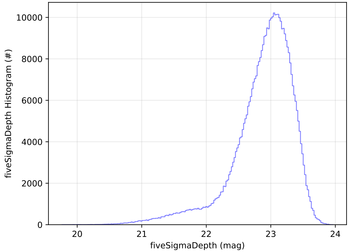
ddf_acor_sf25_lsf40_lsr20_v3.4_10yrs All sky z band: fiveSigmaDepth Histogram
