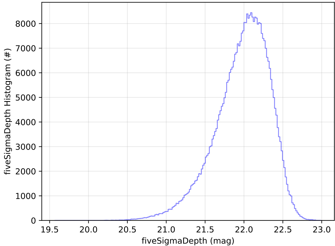
ddf_acor_sf25_lsf40_lsr20_v3.4_10yrs All sky y band: fiveSigmaDepth Histogram
