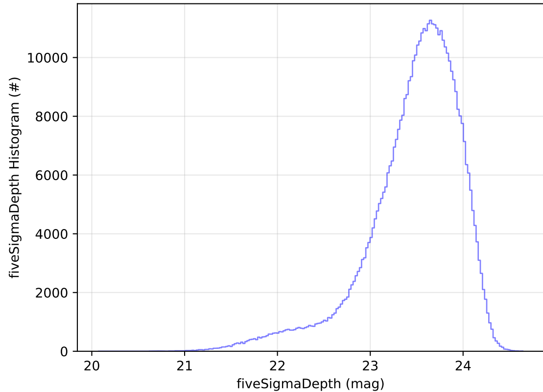
ddf_acor_sf25_lsf40_lsr20_v3.4_10yrs All sky i band: fiveSigmaDepth Histogram
