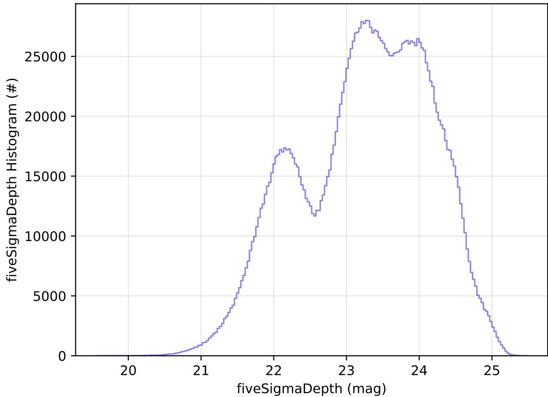
ddf_acor_sf25_lsf40_lsr20_v3.4_10yrs All sky all bands: fiveSigmaDepth Histogram
