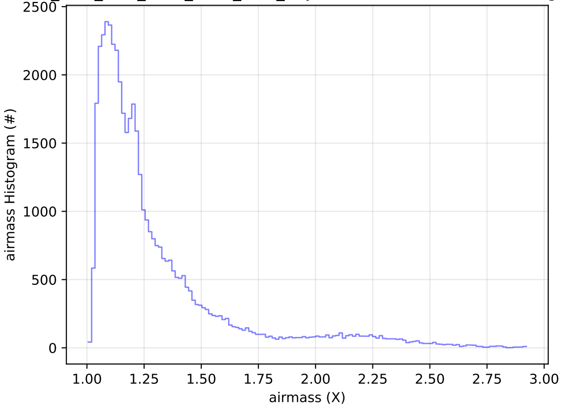
ddf_acor_sf25_lsf40_lsr20_v3.4_10yrs Yr 1 z band: airmass Histogram
